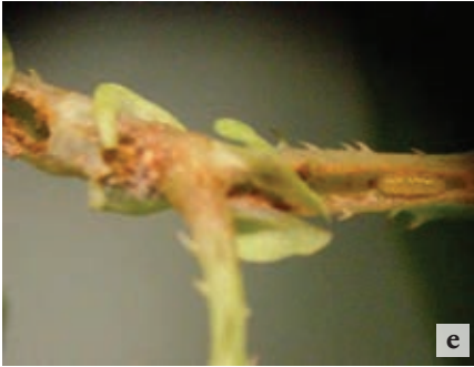
Rhinoncomimus latipes e. larva and damage (Amy Diercks); f. adult feeding damage (Ellen C. Lake, USDA ARS Invasive Plant Research Laboratory)
