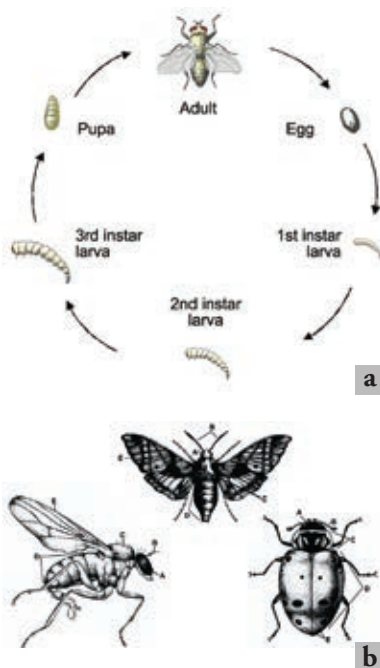
a. Complete metamorphosis of an insect (L. Wilson); b. body parts of adult insects A. head, B. antenna, C. thorax, D. abdomen, E. wing (adapted from Biological Control of Weeds in the West)
