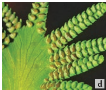
Old World Climbing Fern c. sterile leaflet (left), fertile leaflet (right)(Peggy Greb, USDA ARS); d. fertile leaflet close-up (Amy Ferriter, State of Idaho)(c,d bugwood.org)
