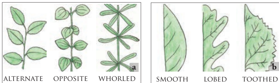
Leaf a. arrangement (how leaves are arranged along a stem); b. margination (shape of a leaf's edges) (a,b Jacqi Sullivan, MIA Consulting)
