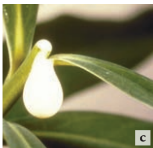
Leafy spurge c. milky latex; d. leaves and stem (K. George Beck & James Sebastian, Colorado State University); e. flowers (c,e Norman E. Rees, USDA ARS)(c-e bugwood.org)
