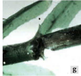
Bagous hydrillae feeding damage (e-g courtesy US Army Corps of Engineers, ERDC-EL)
